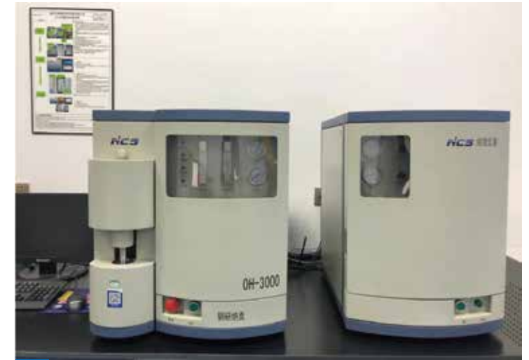
氧氢分析仪 --快速测定钢铁、有色金属、及其它无机材料中氧、氢的含量 NCS Oxygen & Hydrogen Analyzer --Rapid determination of oxygen and hydrogen in steel, non-ferrous metals, and other inorganic materials
